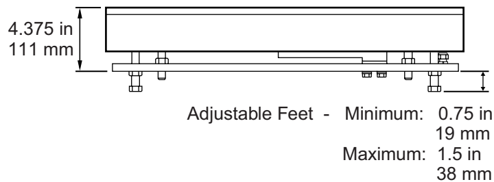
End View
